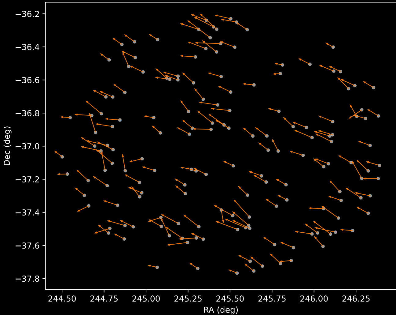
APOGEE DR17 Cluster 2 Proper Motion Vectors (n=158)
