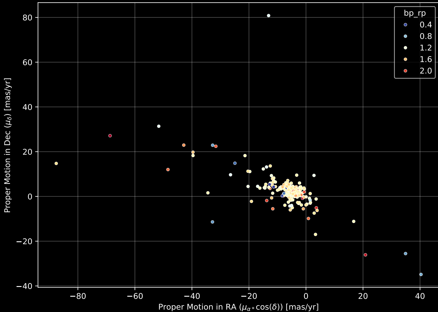
APOGEE DR17 Field: [266+12] Proper Motion Diagram (n= 235)
