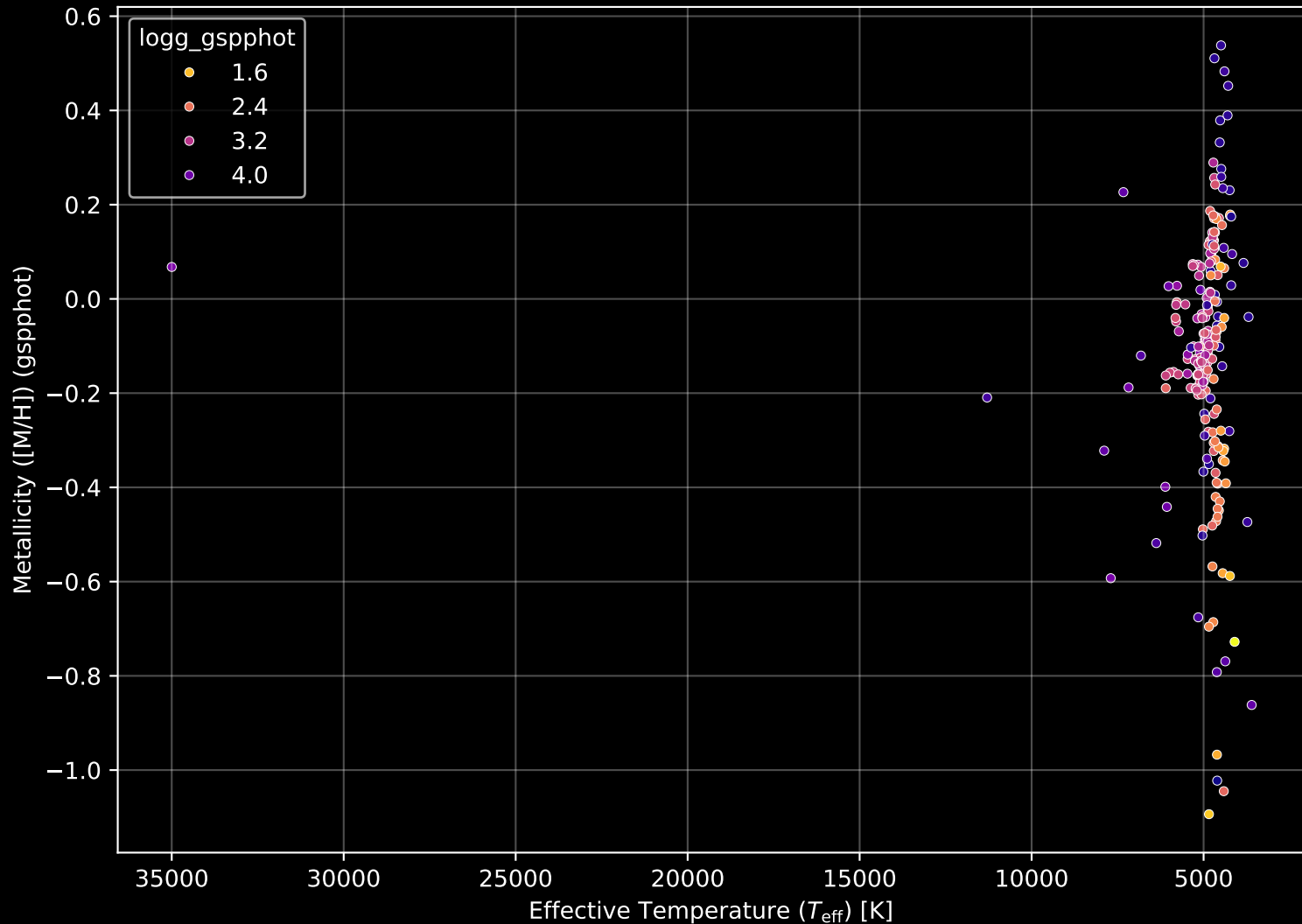
APOGEE DR17 Field: [266+12] Stellar Population Parameters (n= 235)
