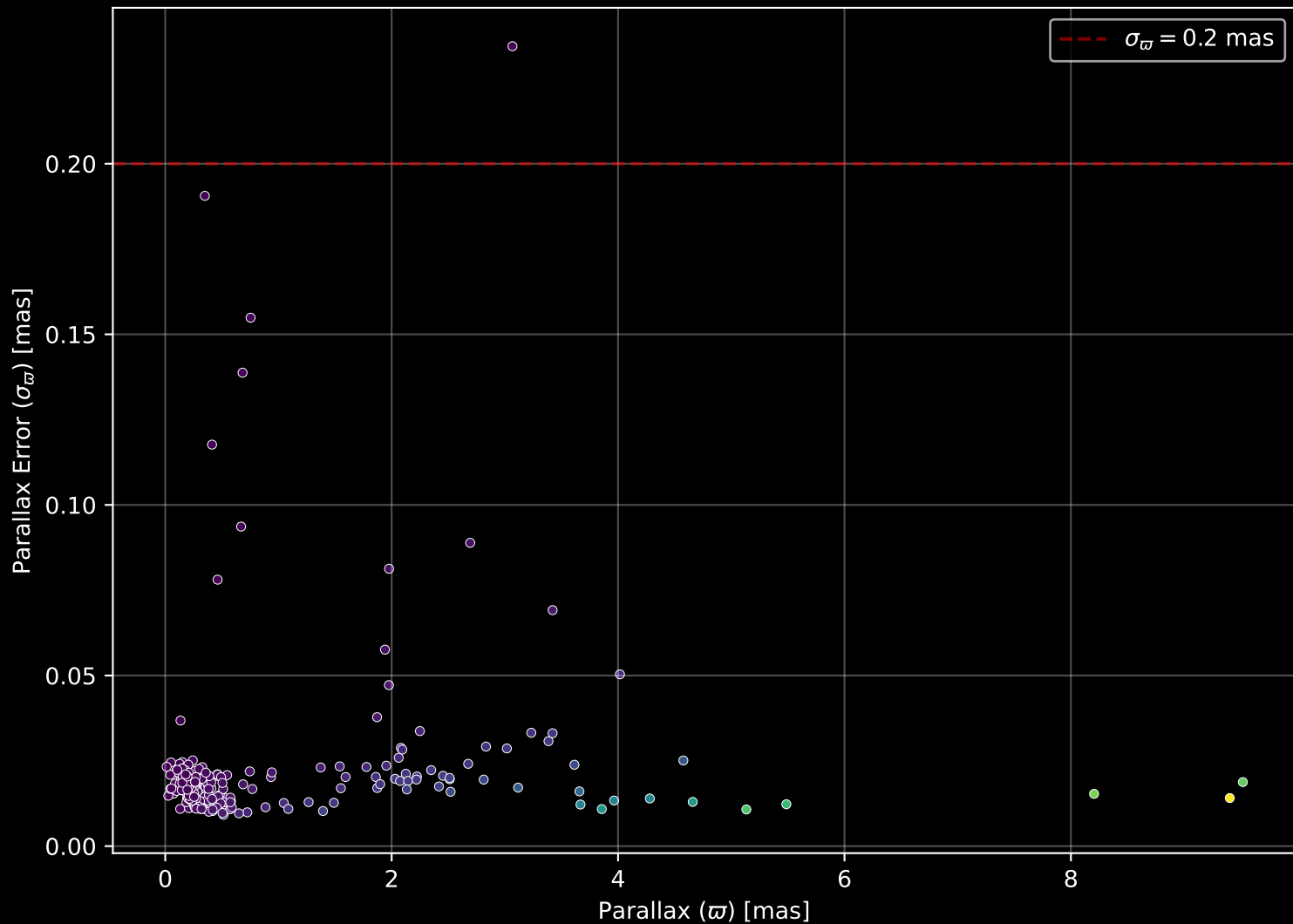
APOGEE DR17 Field: [266+12] Parallax Quality (n= 235)
