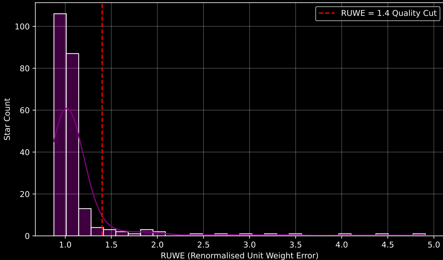
GAPOGEE DR17 Field [266+12] RUWE Distribution (n= 229)
