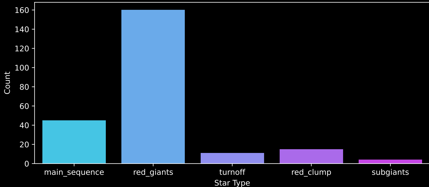
APOGEE DR17 Field: [266+12] Count plot of Star Type
