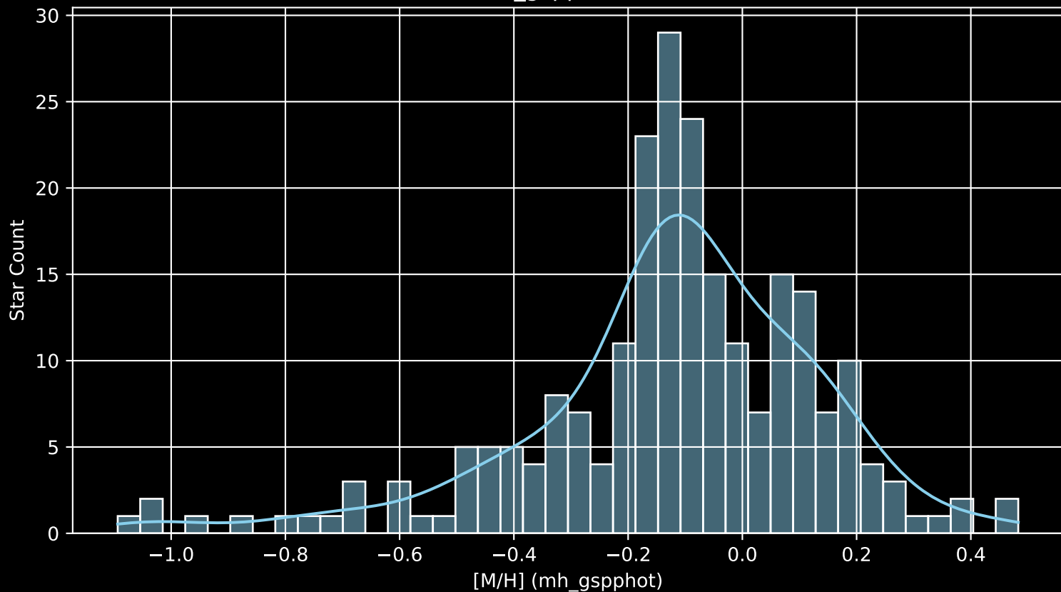
APOGEE DR17 Field: [266+12 [M/H] (mh_gspphot) (n= 233)
